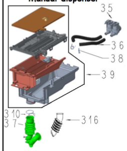
Manual dispenser
