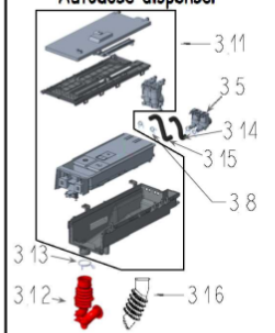
Autodose dispenser
